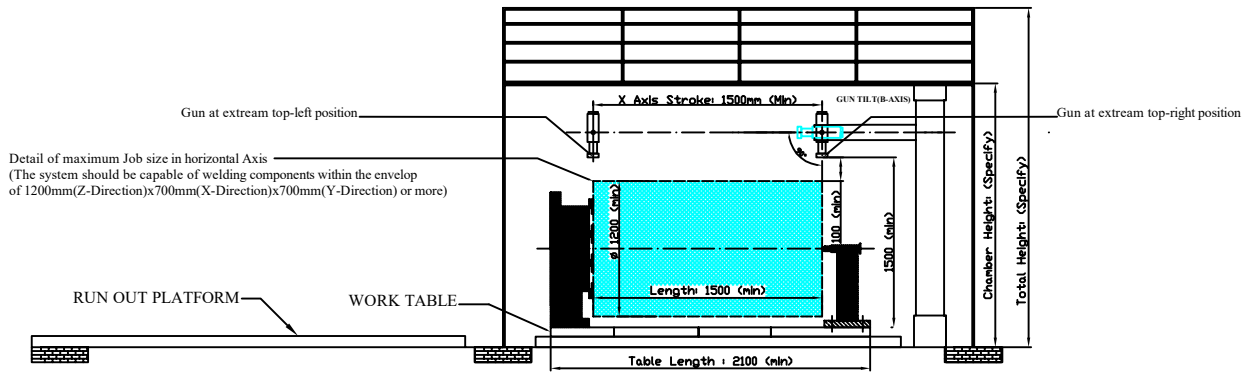
SIDE VIEW-1
