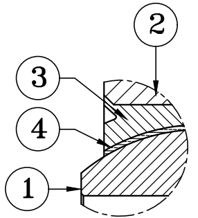
DETAIL-A SCALE-2:1
