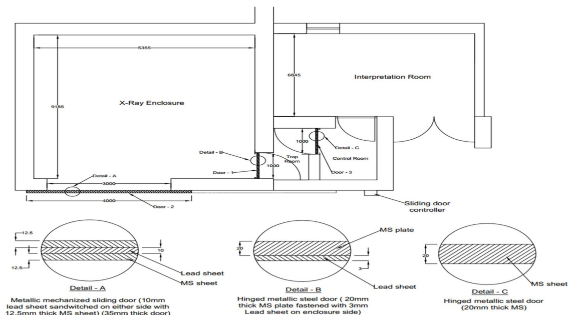
Figure 1 : Schematic diagram of 3 Doors (D1, D2 & D3)—Location & cross sectional detail
