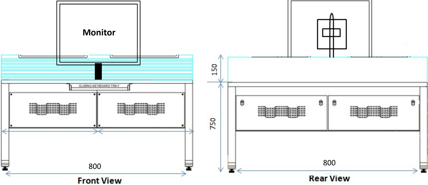
Operator Console (One segment)
